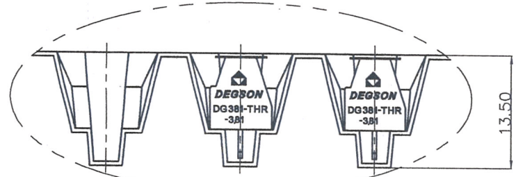
Detail A (2:1)
