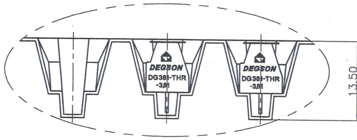
Detail A (2:1)
